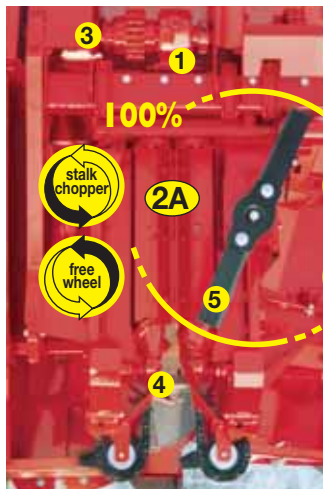
2A Stalk rolls with 5 knives.
