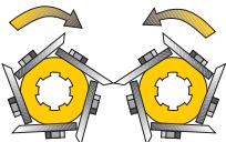
2A Stalk rolls with 5 knives.
